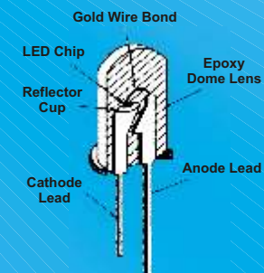
Anatomy of cool white LED
