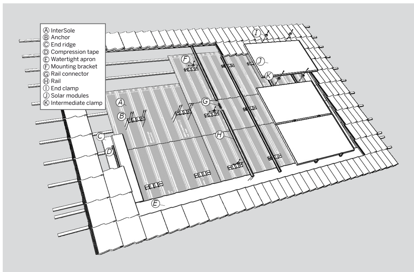
Mounting diagram
